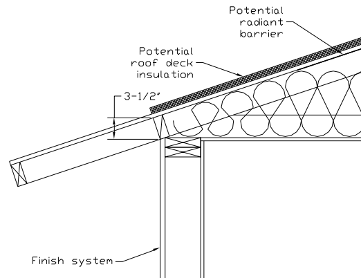
Figure 6-8: Section at Attic Edge with Standard Truss
