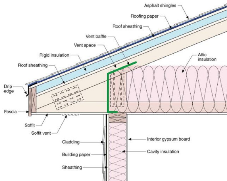
Figure 5-7: Attic with Above Deck Insulation
