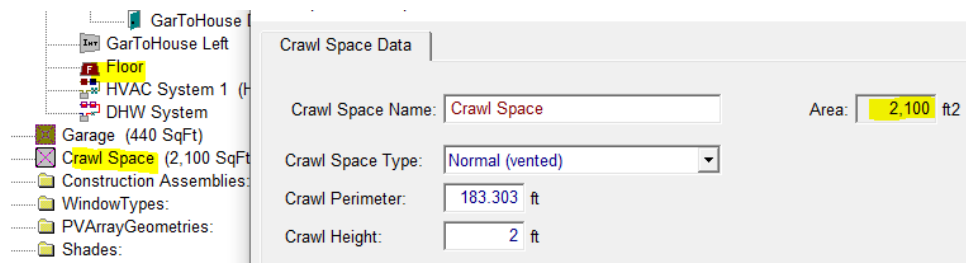
Figure 5-10: Crawl Space Zone
