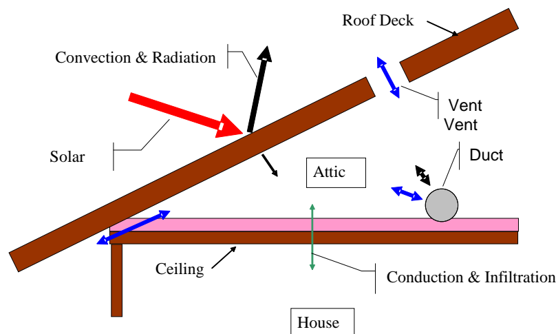
Figure 5-4: Attic Model Components
